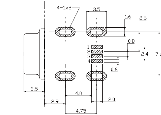
COMPONENT SIDE PCB LAYOUT
